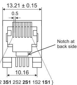
Meter Side RJ 12 Connection
