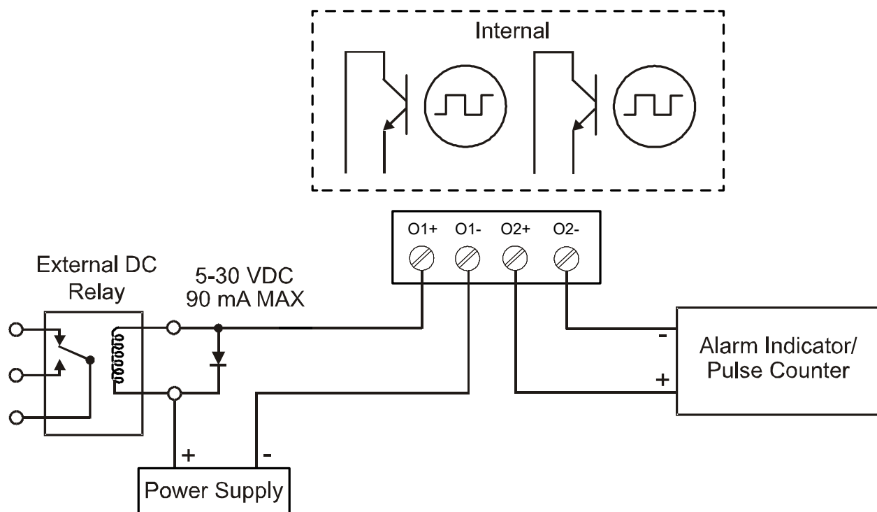
Figure 10. Open Collector Output Connections
