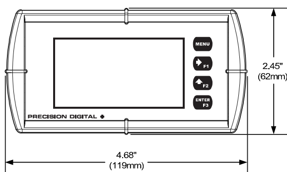
Figure 3. Meter Dimensions - Front View
