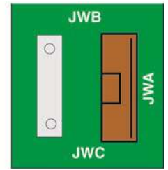
240 VAC Configuration
