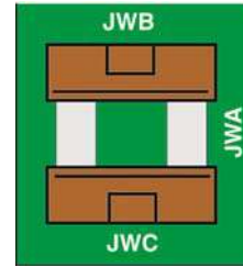
120 VAC Configuration
