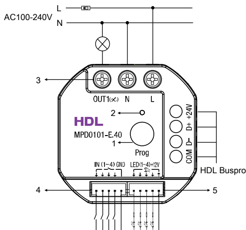
Figure 4. Wiring
