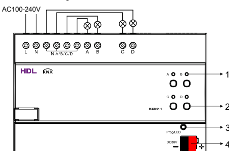
Take the connection of KNX 4CH 1.5A MOSFET Dimming Actuator as an example
