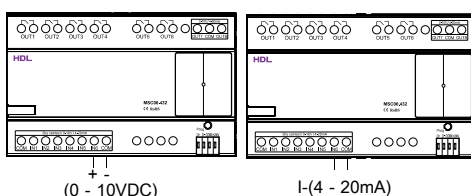
Figure 5. Wiring
