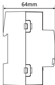
Figure 3. Dimensions-Side View
