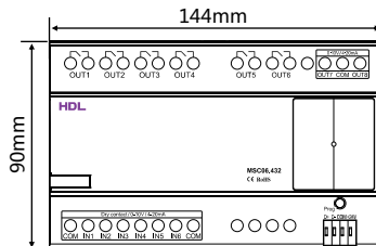
Figure 2. Dimensions-Front View
