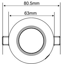
Figure 2. Dimensions - Front View
