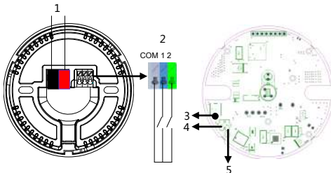
Figure 4. Components - Back View Figure 5. Components - Interior View
