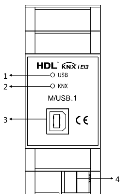
Figure 4. Components - Front View
