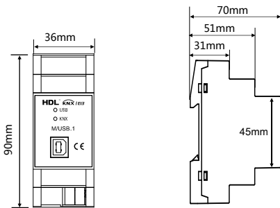
Figure 2. Dimensions - Front View Figure 3. Dimensions - Side View
