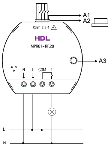
Figure 4. Wiring
