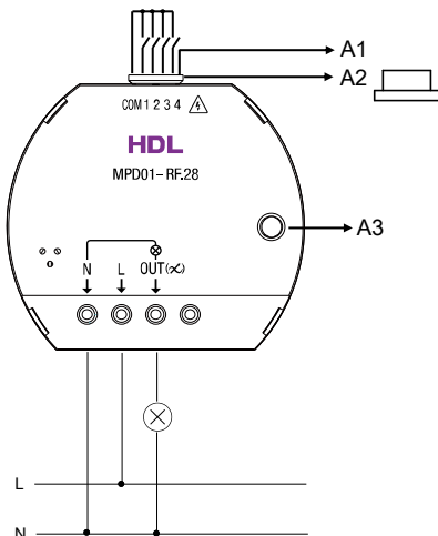
Figure 4. Wiring
