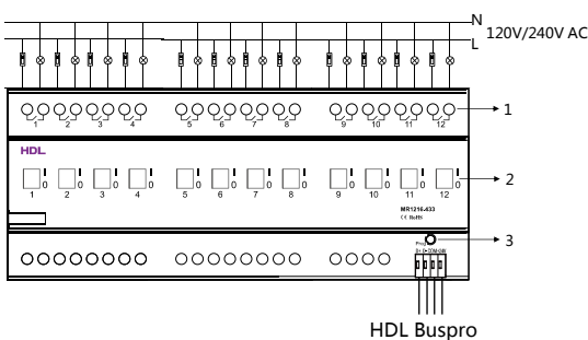
Figure 4. Wiring
