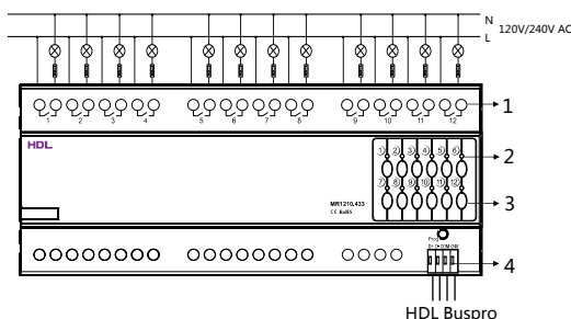
Figure 4. Wiring
