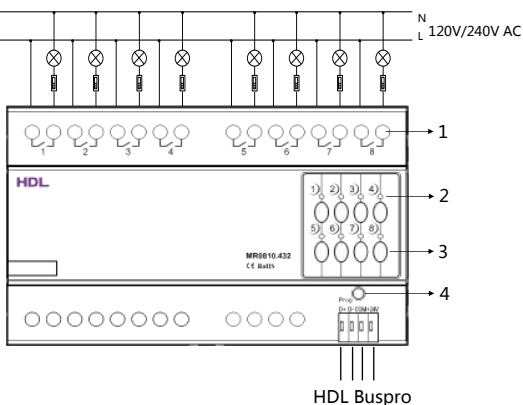
Figure 4. Wiring
