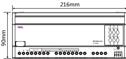
Figure 2. Dimensions - Front View
