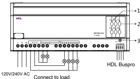
Figure 4. Wiring
