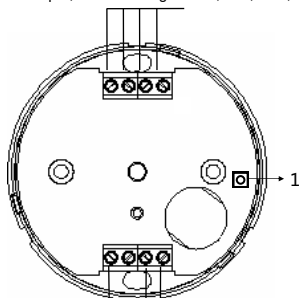
Figure 6. Wiring
